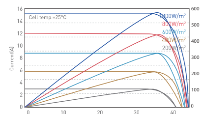
I-V curves/P-V curves at different irradiance (570W)
