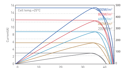
I-V curves/P-V curves at different irradiance (435W)
